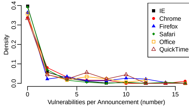
Figure 4: Histogram of vulnerabilities announced on announcement day.
