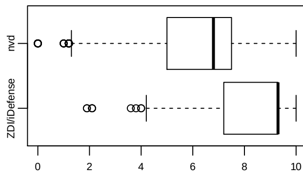
Figure 13: Distribution of CVSS scores: NVD versus ZDI/iDefense.
