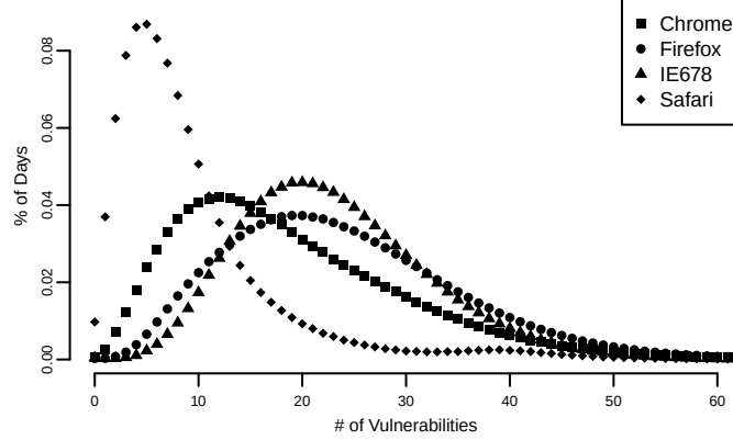
Figure 6: Percent of days with the given number of vulnerabilities in a vendors queue
