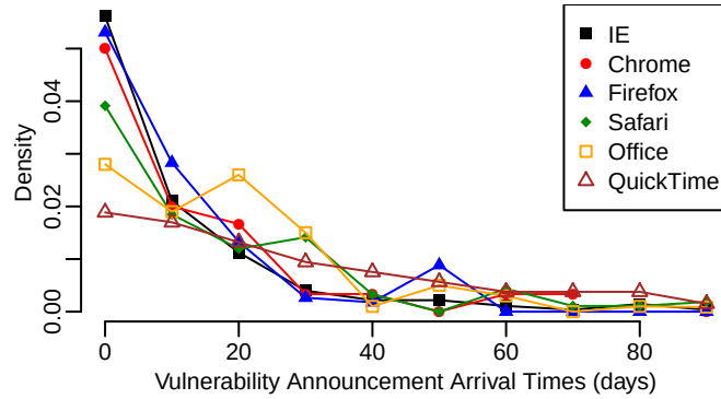
Figure 3: Histogram of vulnerability announcement rates.
