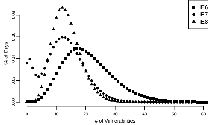
Figure 7: Days with given number of vulnerabilities (MS IE)
