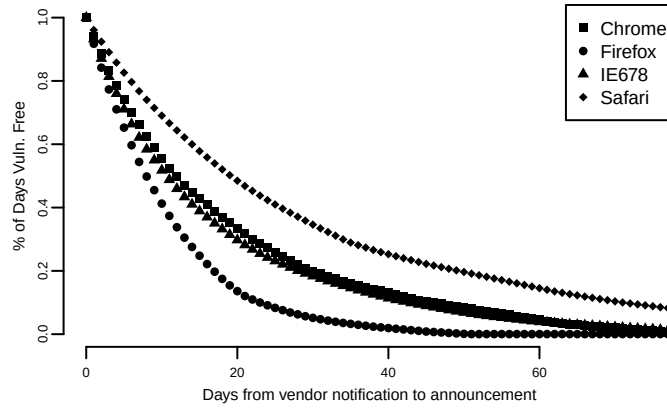
Figure 8: Vulnerability Free Days (VFD), as a function of lifespans
