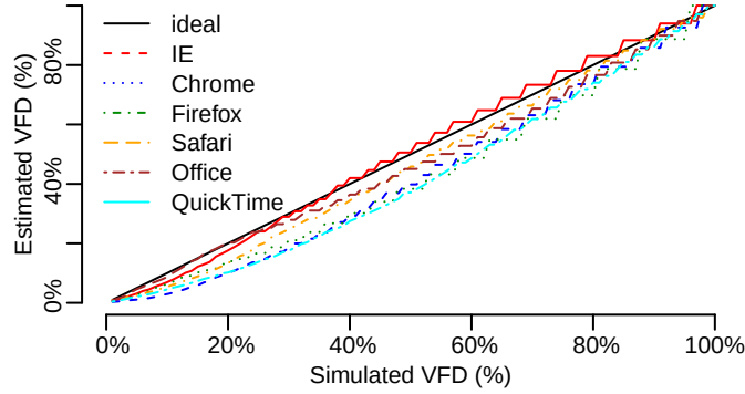
Figure 11: Estimation of VFD metric using shortcut formula
