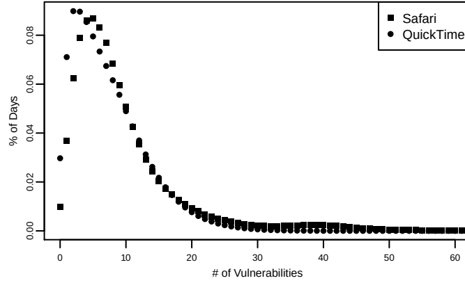
Figure 9: Comparison of Microsoft Products
