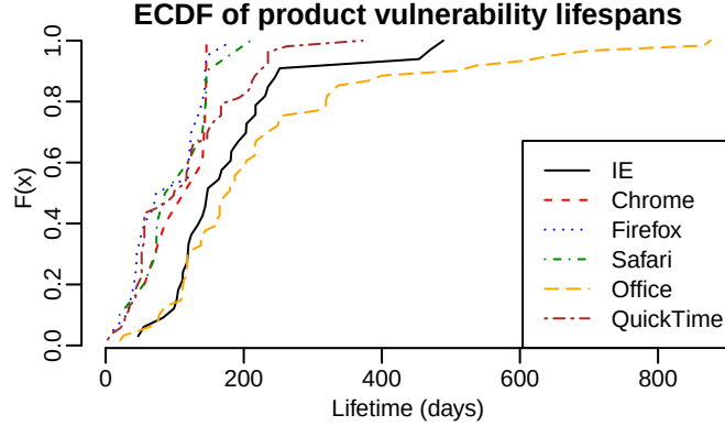
Figure 5: Empirical cumulative distribution functions of product vulnerability lifespans.
