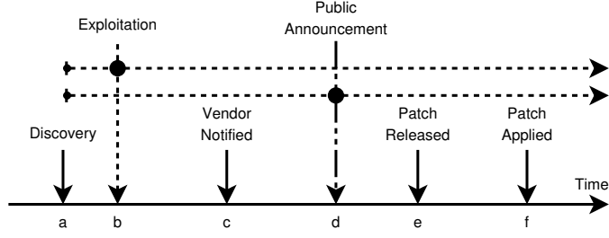
Figure 1: Vulnerability lifetime model
